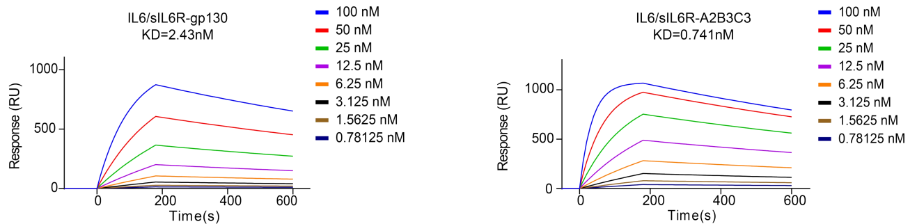
Figure 1. Representative surface plasmon resonance (SPR) sensorgrams showing the binding of (A) gp130 and (B) A2B3C3 to the immobilized IL-6/sIL-6R \alpha complex at the indicated concentrations (0.78125-100 nM). Kinetic fitting yielded equilibrium dissociation constants ( K_D ) of 2.43 nM for gp130 and 0.741 nM for A2B3C3.
